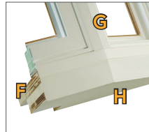
F. Insulated seat board with 3/4" exterior clad plywood. Super Seat Dow® Foam 3" thick sandwich with R-9 performance for thermal protection and fight condensation.
