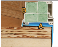
A. Exclusive welded sill pan (blue) eliminates water penetration and provides a built-in weep system with a smooth finish on the exterior surface of the seat board.
