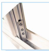
Strong Metal Reinforcement - Stainless steel L brackets at keeper rail connect to the L channel in the mainframe head and sill as well as the external keeper rail reinforcement for extra durability and protection during violent weather.
