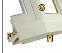
F. Insulated seat board with 3/4" exterior clad plywood. Super Seat Dow® Foam 3" thick sandwich with R-9 performance for thermal protection and fight condensation.
